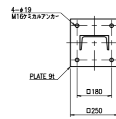
BASE PLATE [-150]
