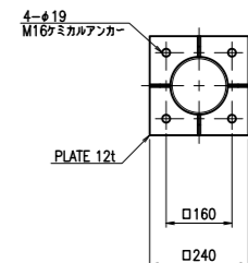
BASE PLATE 125A
