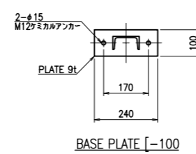
BASE PLATE [-100-2]
