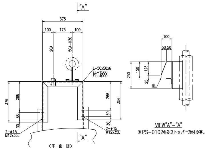
PS-0101 EL+1500 PS-0102 EL+4000
