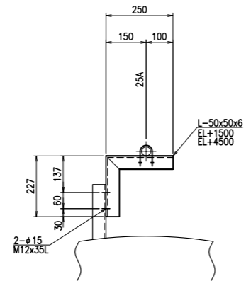
PS-0119 EL+1500 PS-0120 EL+4500
