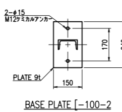
BASE PLATE [-100]
