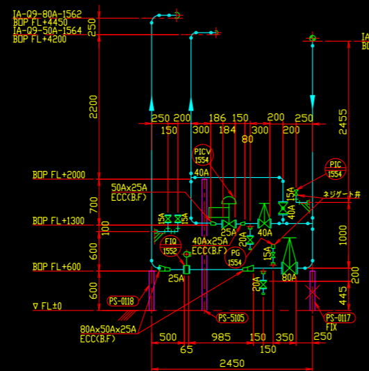
VIEW "G" - "G"
