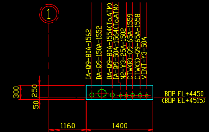
VIEW "J" - "J"
