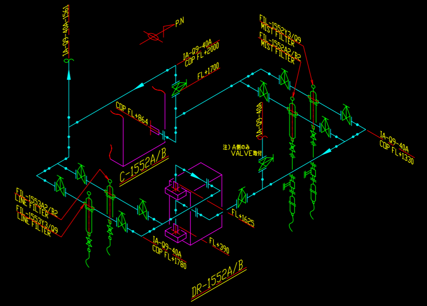
DETAIL "I"
