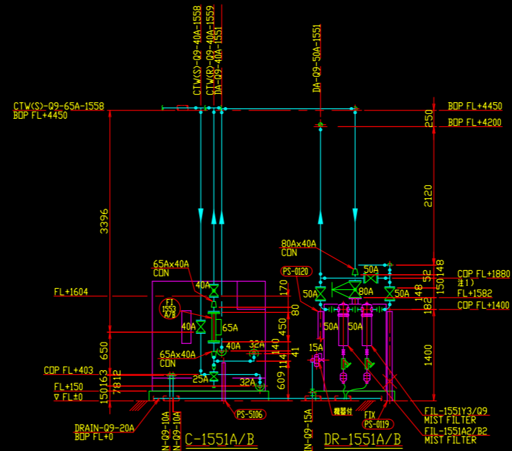
VIEW "B" - "B"
