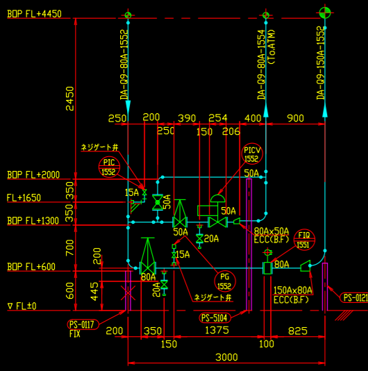
VIEW "F" - "F"
